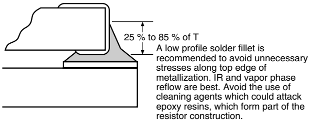
FIGURE 4 - RECOMMENDED MOUNTING
