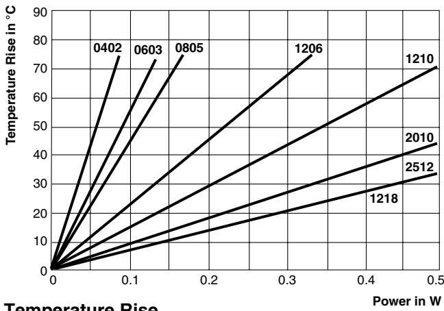
Temperature Rise
