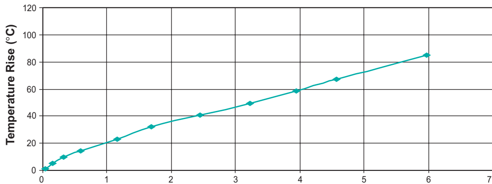
Temperature Rise vs. Power (W) Dissipation
