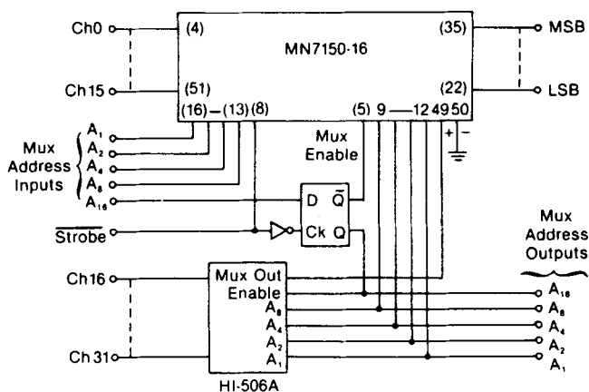
Expansion to 32 Single-ended Channels
