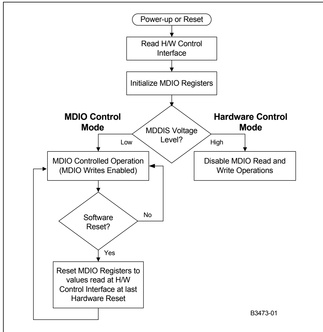
Figure 7 Initialization Sequence
