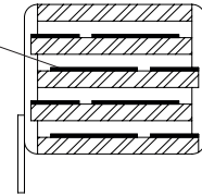
3 sections (2000Vdc)
