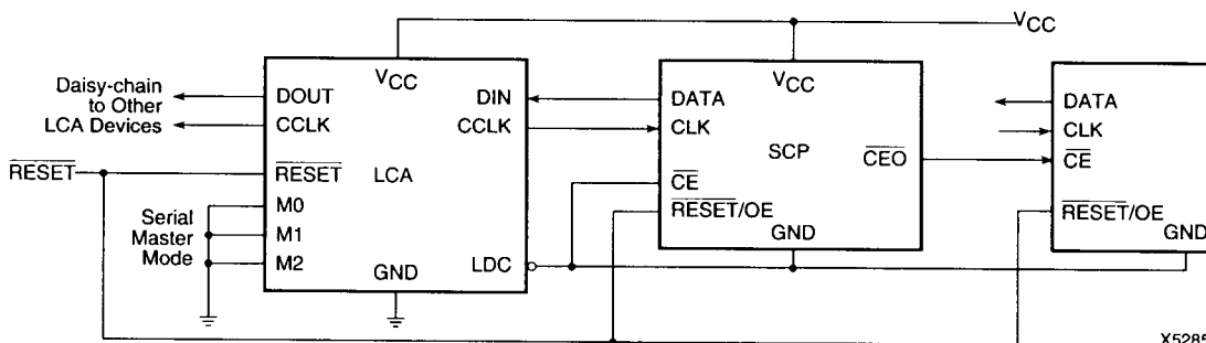
Figure 4. Zero-Standby Current Circuit
