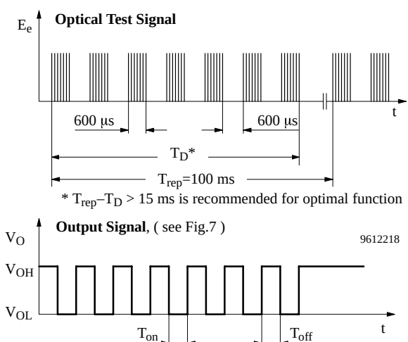
Figure 6. Output Function
