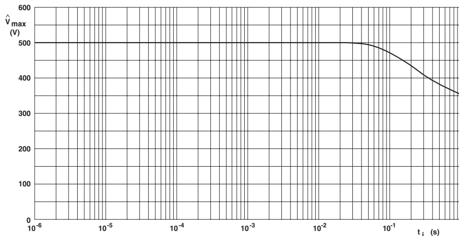
SFR25 Pulse on a regular basis; maximum permissible peak pulse voltage ( \hat{V}_{max} ) as a function of pulse duration ( t_i )
