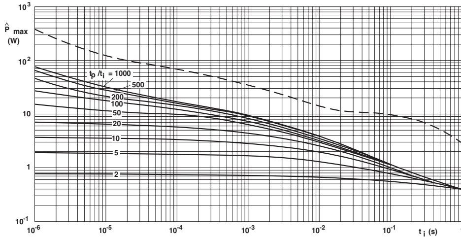
SFR25 Pulse on a regular basis; maximum permissible peak pulse power ( \hat{P}_{max} ) as a function of pulse duration ( t_i )
