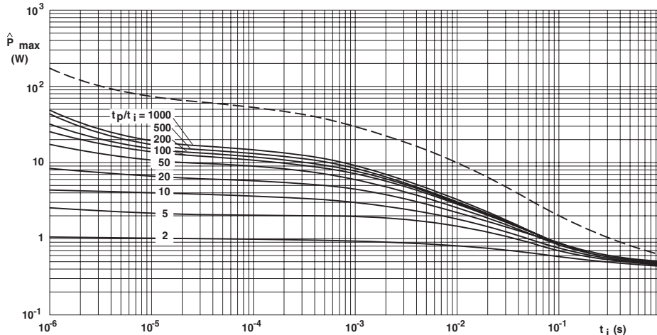
SFR16S Pulse on a regular basis; maximum permissible peak pulse power ( \hat{P}_{max} ) as a function of pulse duration ( t_i )
