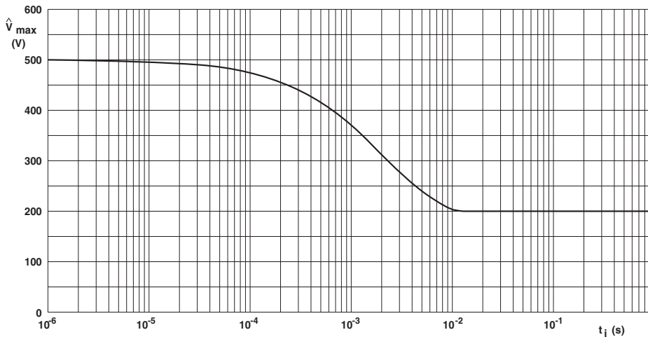
SFR16S Pulse on a regular basis; maximum permissible peak pulse voltage ( \hat{V}_{max} ) as a function of pulse duration ( t_i )
