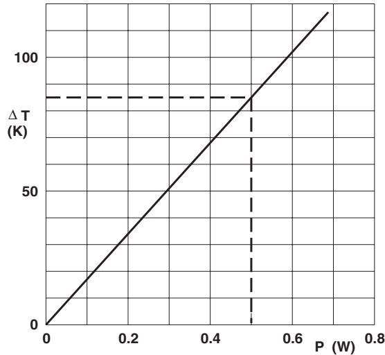
SFR16S Hot-spot temperature rise ( \Delta T ) as a function of dissipated power
