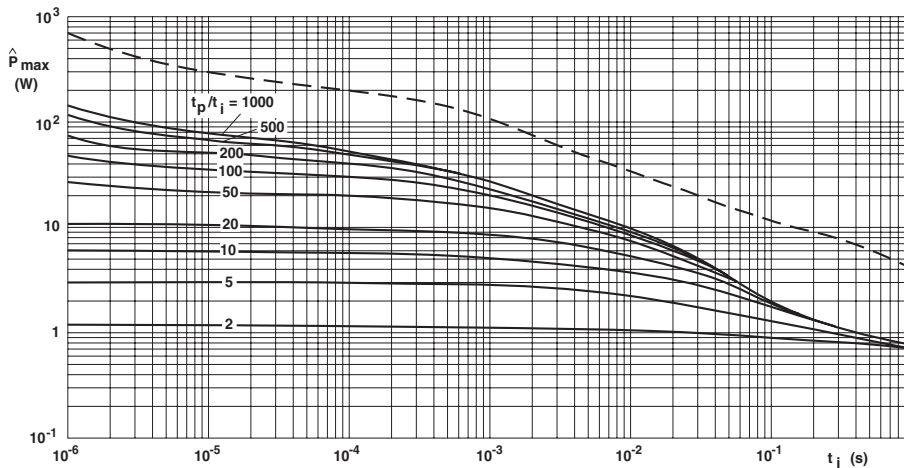
SFR25H Pulse on a regular basis; maximum permissible peak pulse power ( \hat{P}_{max} ) as a function of pulse duration ( t_i )
