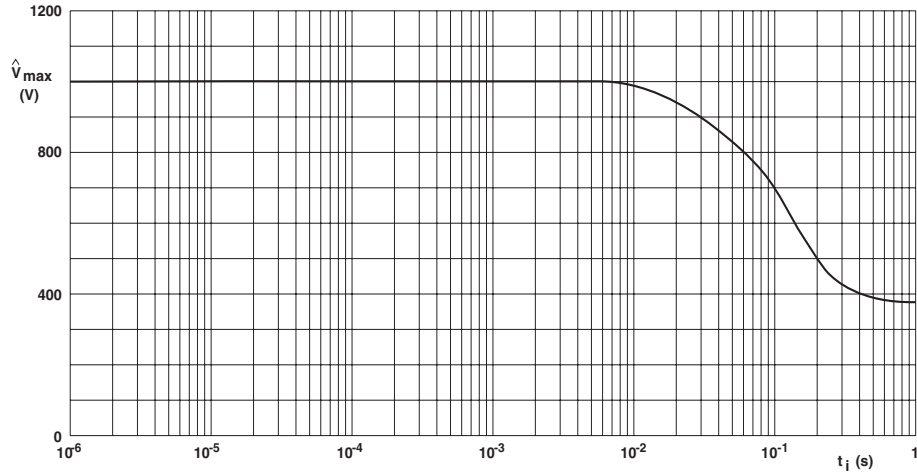
SFR25H Pulse on a regular basis; maximum permissible peak pulse voltage ( \hat{V}_{max} ) as a function of pulse duration ( t_i )
