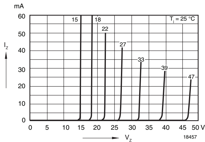
Figure 8. Breakdown Characteristics
