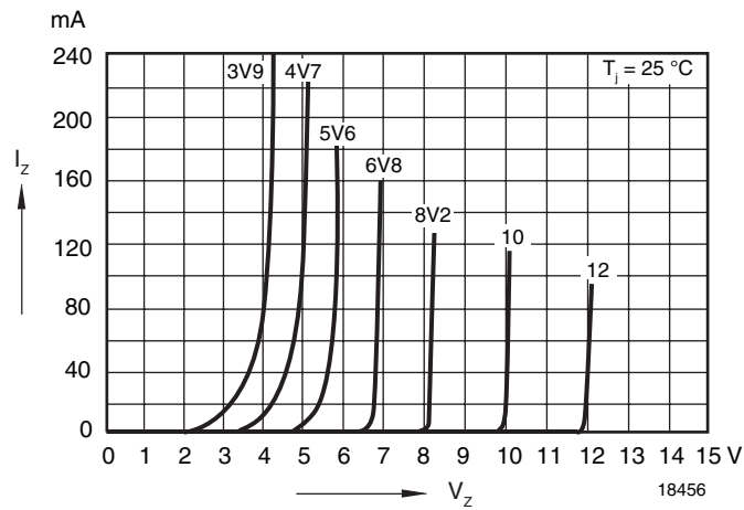
Figure 7. Breakdown Characteristics
