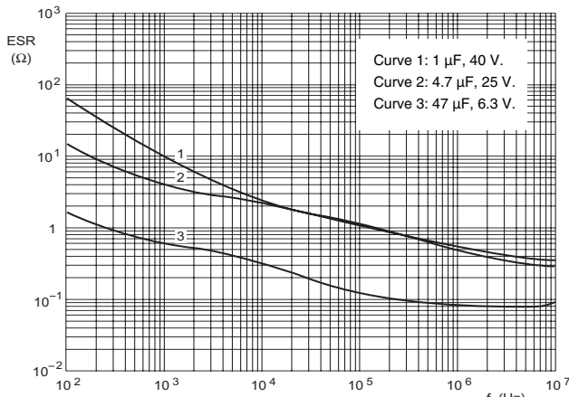
Fig.16 Typical ESR as a function of frequency.
