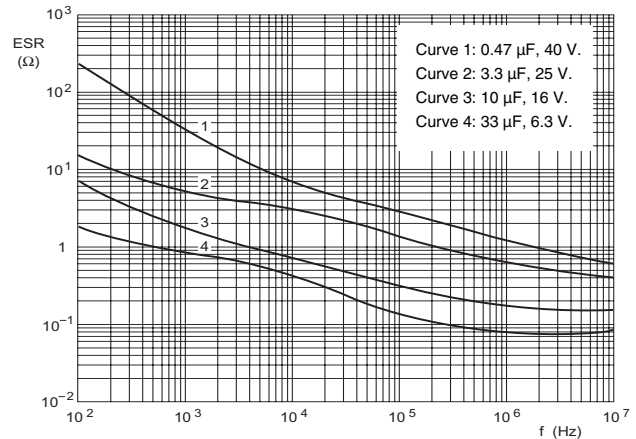
Fig.15 Typical ESR as a function of frequency.
