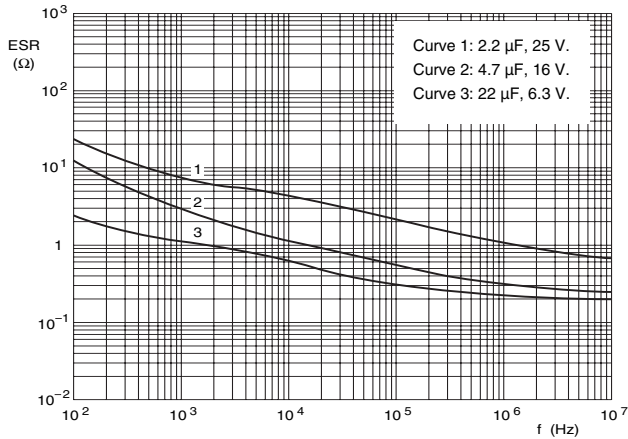
Fig.14 Typical ESR as a function of frequency.
