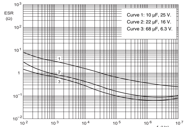
Fig.17 Typical ESR as a function of frequency.
