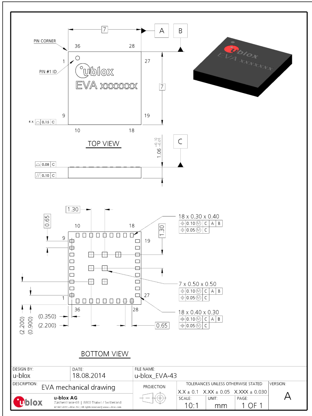
Figure 4: Mechanical drawing for EVA-M8M (LGA43)
