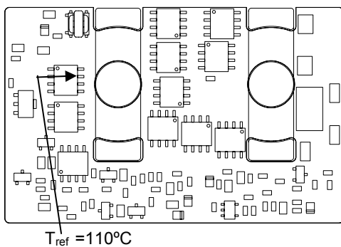
Figure 39. T_{ref} Temperature Measurement Location for V_o=1.8V .
