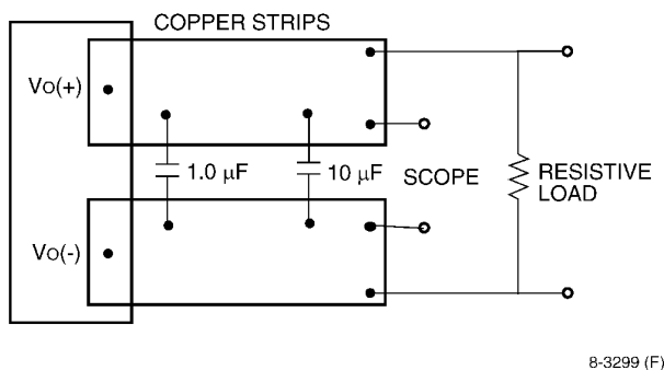
Figure 31. Input Reflected Ripple Current Test Setup.
