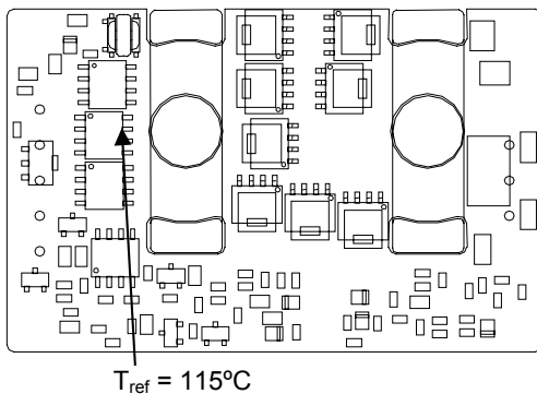
Figure 38. T_{ref} Temperature Measurement Location for V_o=3.3V - 2.5V .
