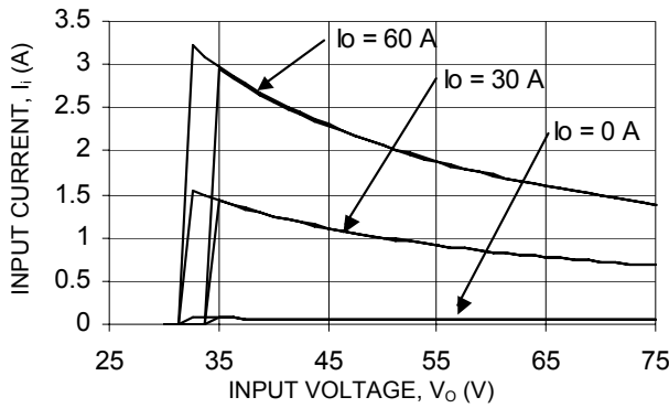
Figure 19. Typical Input Characteristic at Room Temperature.
