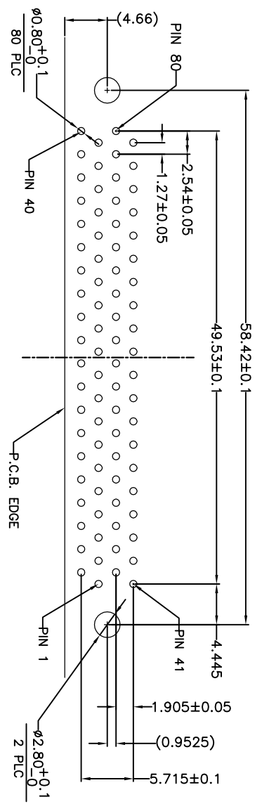
RECOMMENDED PC BOARD LAYOUT
