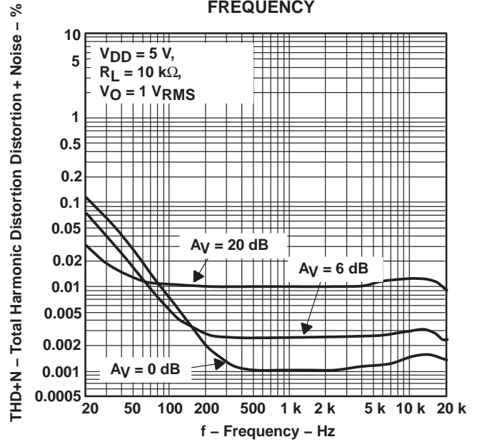
HEADPHONE TOTAL HARMONIC DISTORTION + NOISE VS FREQUENCY
