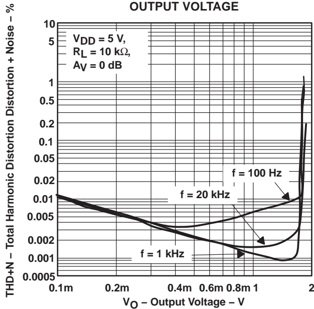
HEADPHONE TOTAL HARMONIC DISTORTION + NOISE VS OUTPUT VOLTAGE
