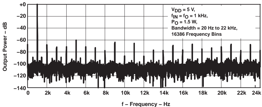
FFT AT 1.5-W OUTPUT POWER vs FREQUENCY
