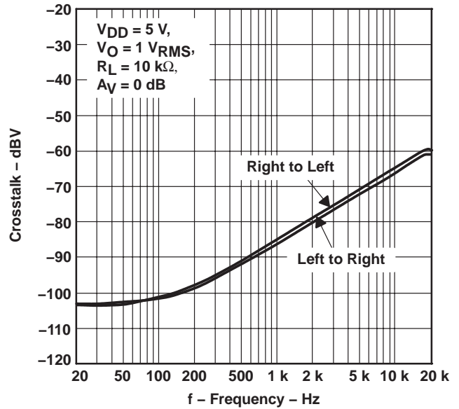
HEADPHONE CROSSTALK VS FREQUENCY
