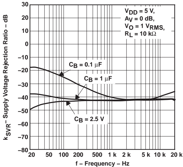
HEADPHONE SUPPLY VOLTAGE REJECTION RATIO VS FREQUENCY
