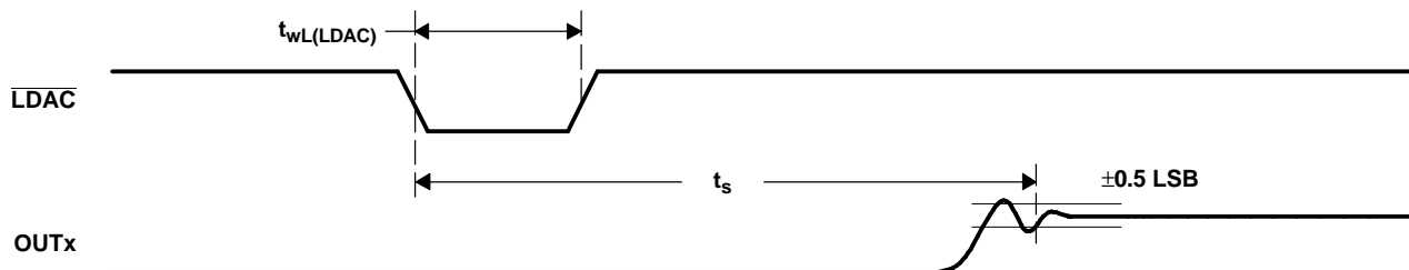
Figure 12. Output Timing
