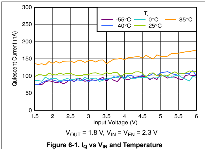
Figure 6-1. I_Q vs V_{IN} and Temperature
