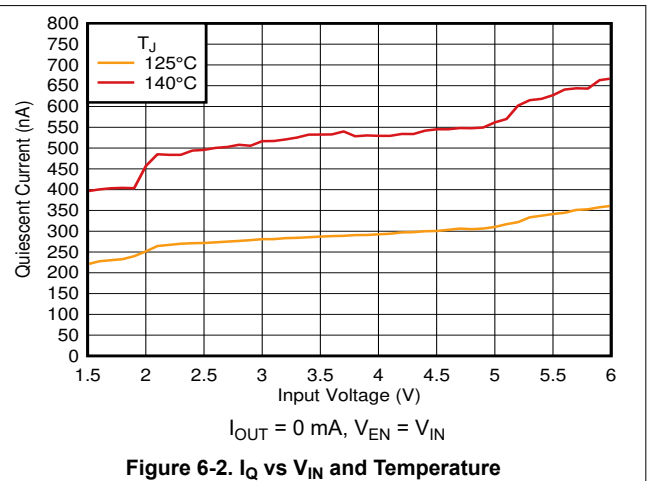
Figure 6-2. I_Q vs V_{IN} and Temperature
