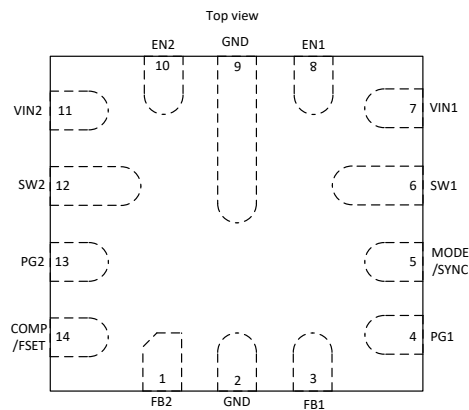
Figure 6-1. 14-Pin VQFN-HR RQR Package
