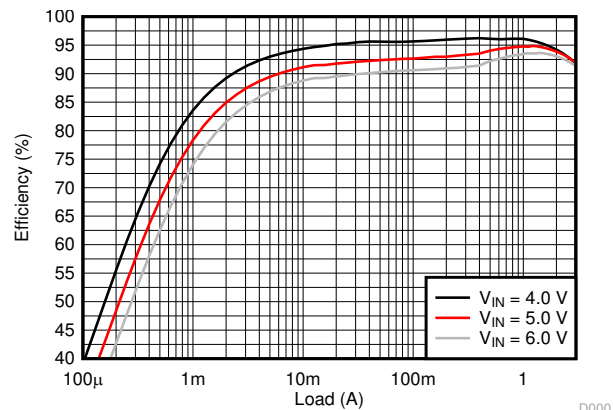
Efficiency vs Output Current, V_{OUT} = 3.3\text{ V} , PWM and PFM, f_{SW} = 2.25\text{ MHz}
