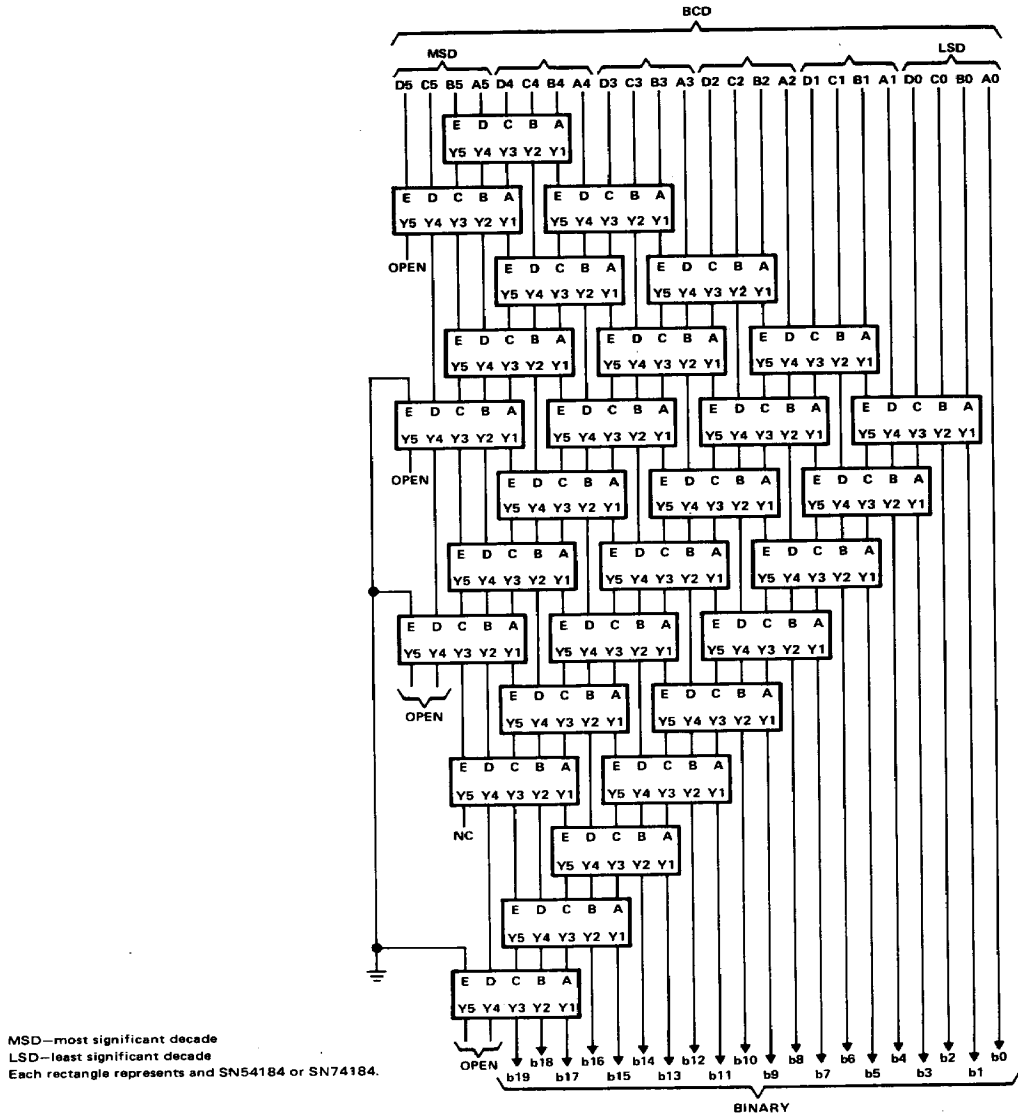
FIGURE 4—BCD-TO-BINARY CONVERTER FOR SIX BCD DECADES
