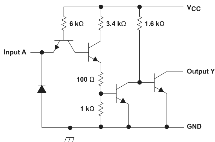
Figure 3. Schematic
