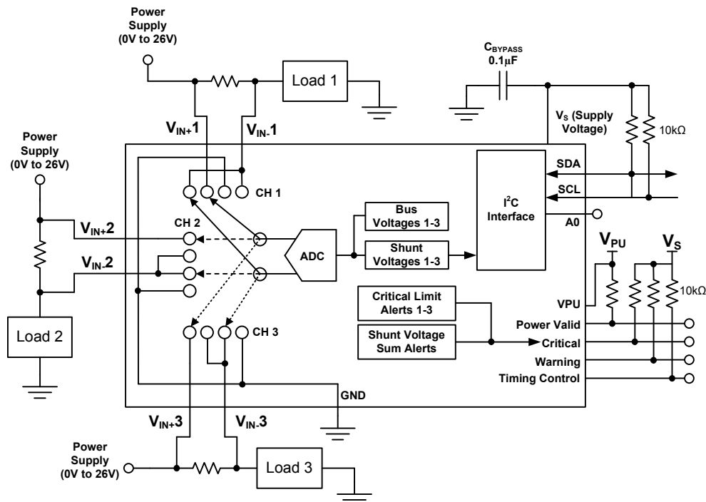
Figure 20. Typical Application Diagram
