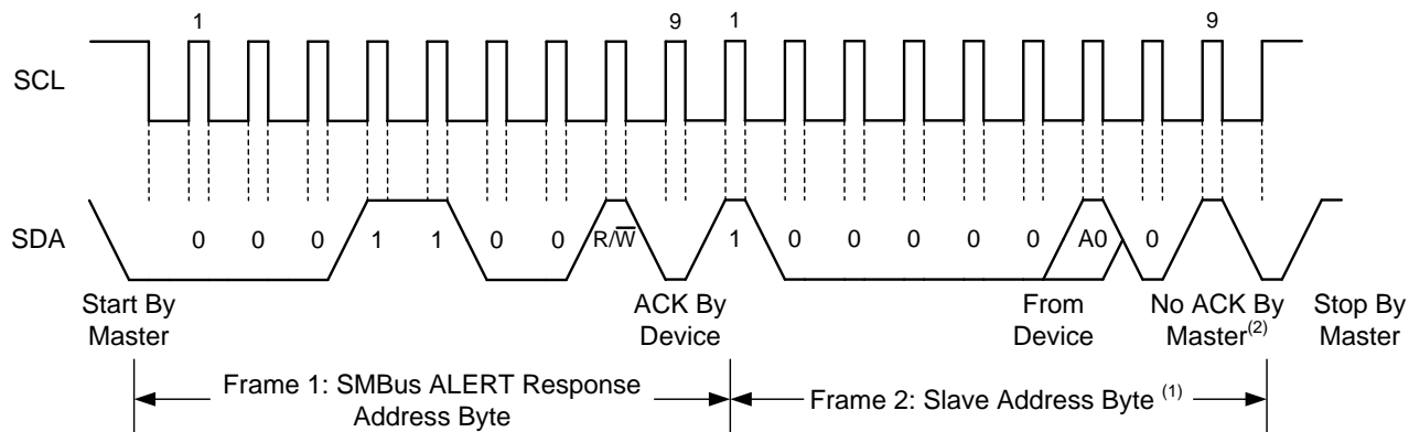
Figure 31. Timing Diagram for SMBus ALERT
