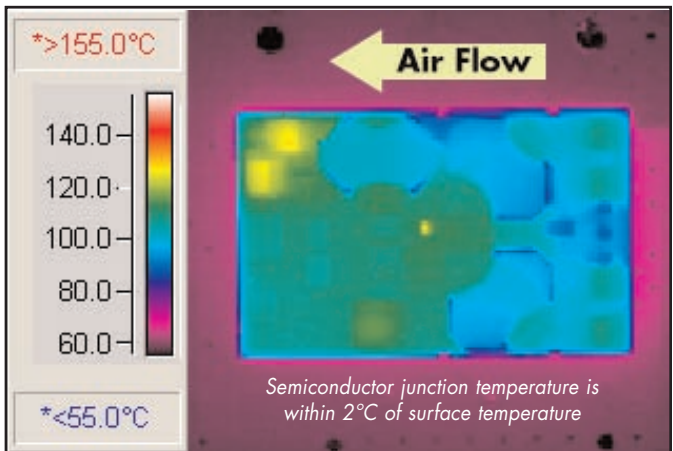
Figure 8: Thermal plot of converter at 23.4 amp load current with 55°C air flowing at the rate of 200 LFM. Air is flowing across the converter in the long direction from output to input (nominal input voltage).
