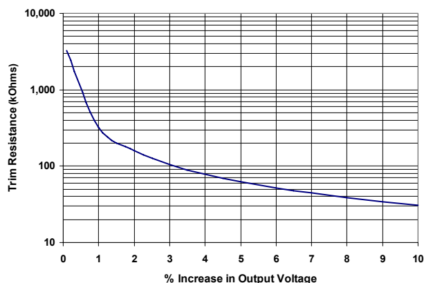
Figure C: Trim Up Graph for 2.0V out
