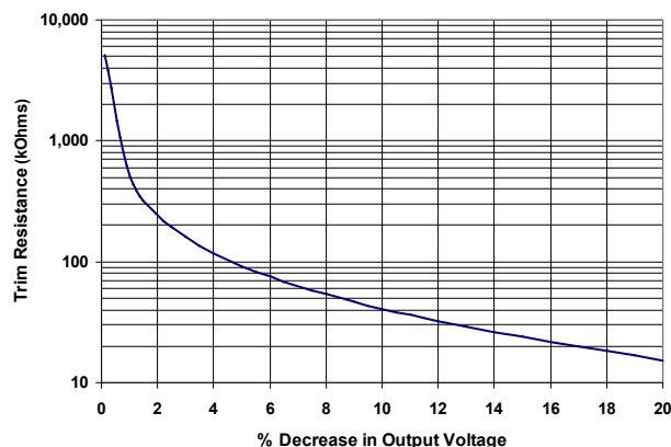
Figure B: Trim Down Graph for 2.0V out
