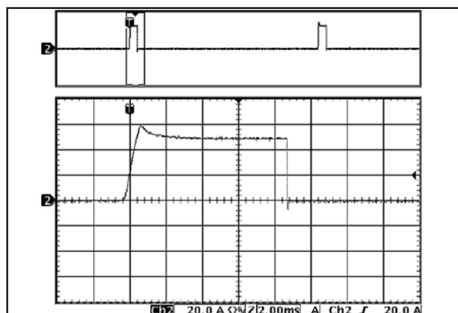
Figure 18: Load current (20 A/div) as a function of time when the converter attempts to turn on into a 1\ \text{m}\Omega short circuit. Bottom trace (2 ms/div) is an expansion of the on-time portion of the top trace.
