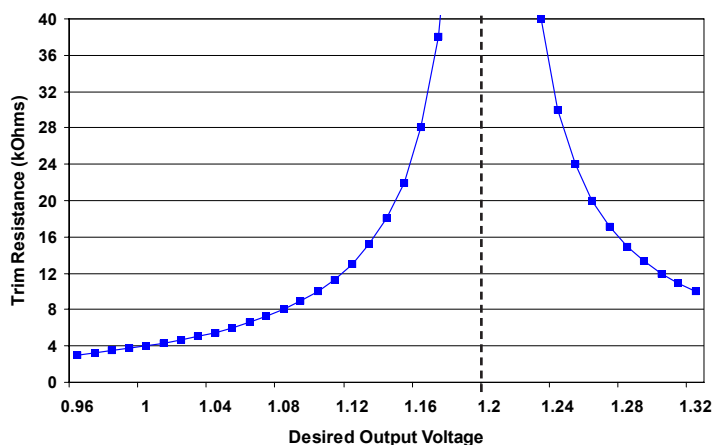
Figure C: Trim Graph for 1.2Vout module
