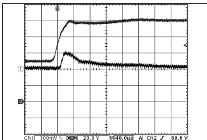
Figure 17: Output voltage response to step-change in input voltage (50V to 100V in 40 μs). Load cap: 10\ \mu\text{F} , 100\ \text{m}\Omega ESR tantalum capacitor and 1\ \mu\text{F} ceramic cap. Ch 1: V_{out} (100 mV/div), Ch 2: V_{in} (20 V/div).
