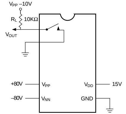
T_{ON}/T_{OFF}
