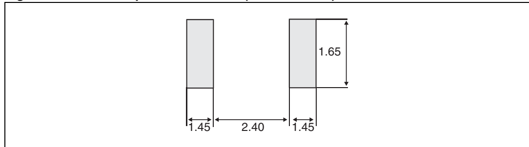
Figure 18. SMA footprint dimensions (in millimeters)
