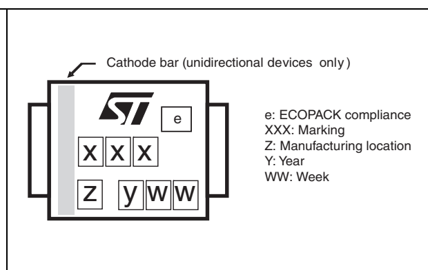
Figure 14. Marking layout (1)
