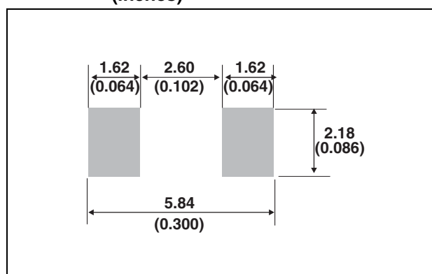
Figure 13. SMB footprint dimensions in mm (inches)
