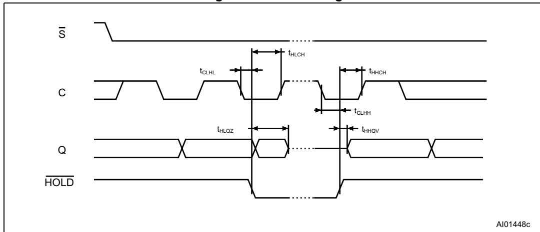
Figure 19. Hold timing
