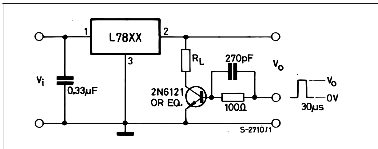
Figure 2 : Load Regulation
