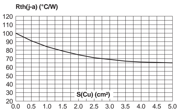
Fig. 9-1: Thermal resistance junction to ambient versus copper surface under each lead (Epoxy printed circuit board FR4, copper thickness: 35 \mu m ) (SMB).
