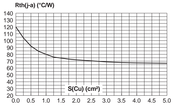
Fig. 9-2: Thermal resistance junction to ambient versus copper surface under each lead (Epoxy printed circuit board FR4, copper thickness: 35 \mu m ) (SMA).
