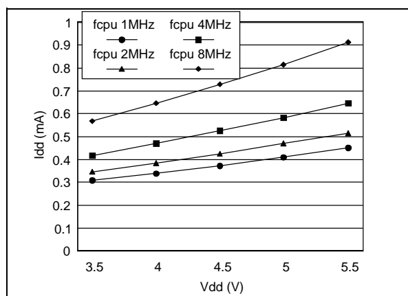
Figure 124. Typical I_{DD} in SLOW-WAIT vs. f_{OSC}
