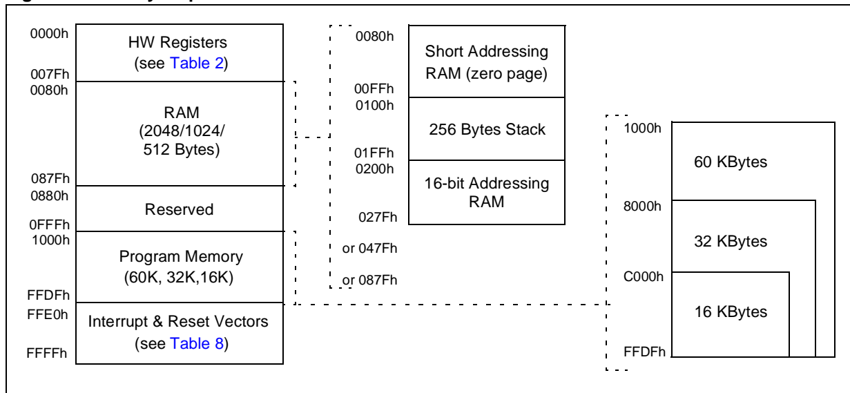
Figure 5. Memory Map
