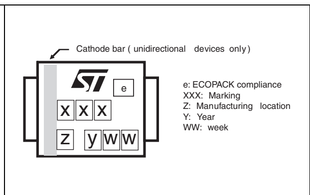
Figure 14. Marking layout (1)
