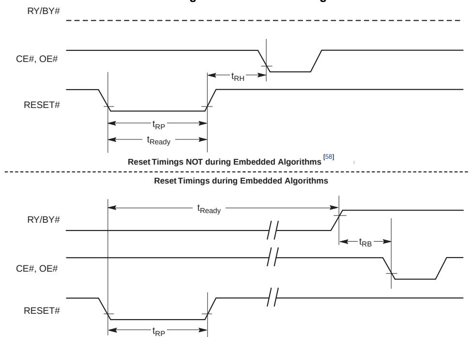
Figure 16. RESET# Timings
