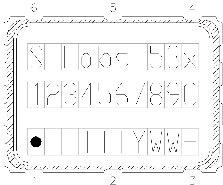
Figure 5. Mark Specification
