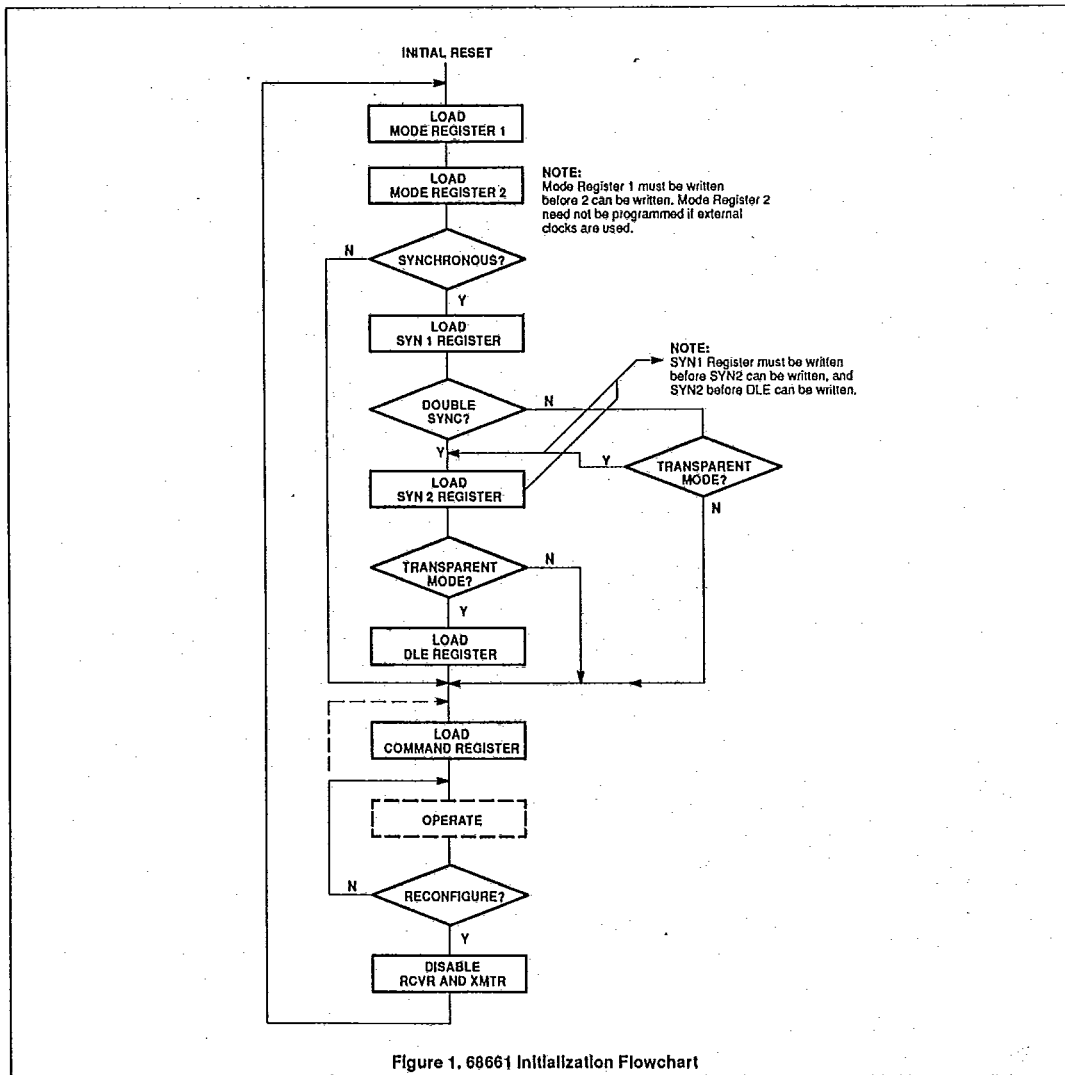
Figure 1. 68661 Initialization Flowchart
