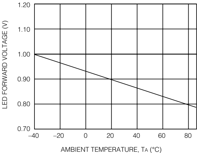
B. LED Dropout Voltage vs. Temperature
