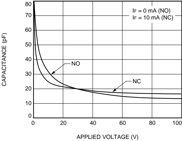
F. Switch Capacitance vs. Applied Voltage
