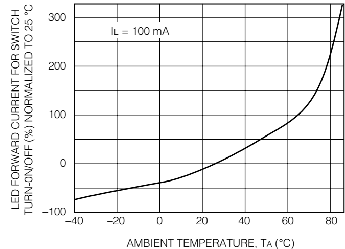
C. LED Current for Switch Turn-On/Off vs. Temperature
