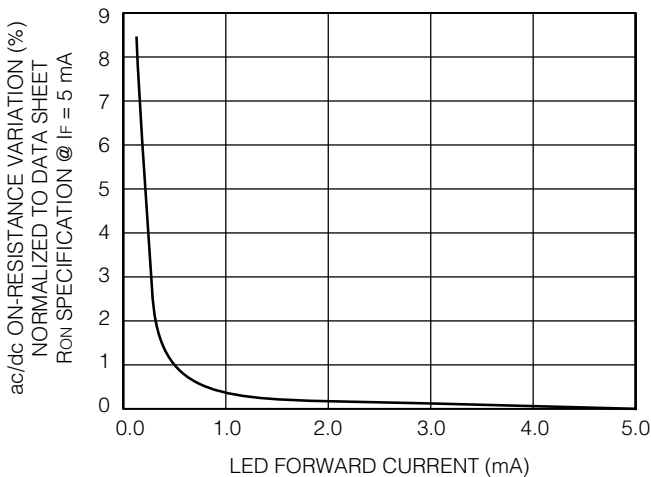
F. Variation in ON-Resistance vs. LED Current
