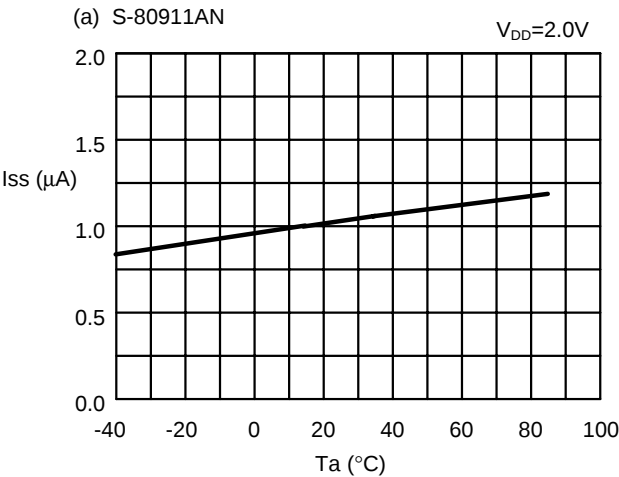
(4) Current consumption ( I_{SS} ) - Temperature ( T_a )
