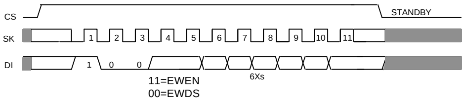
Figure 20 EWEN/EWDS Timing (S-93C56A)
