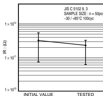
Fig.15 Insulation resistance
