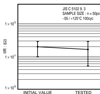
Fig.12 Insulation resistance
