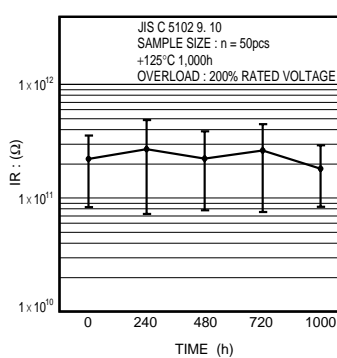
Fig.21 Insulation resistance
