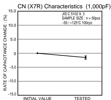
Fig.10 Rate of capacitance change
