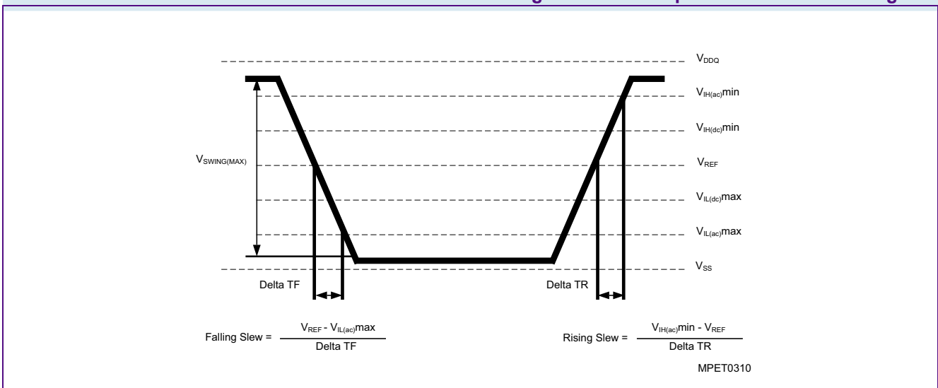
FIGURE 3 Single-ended AC Input Test Conditions Diagram
