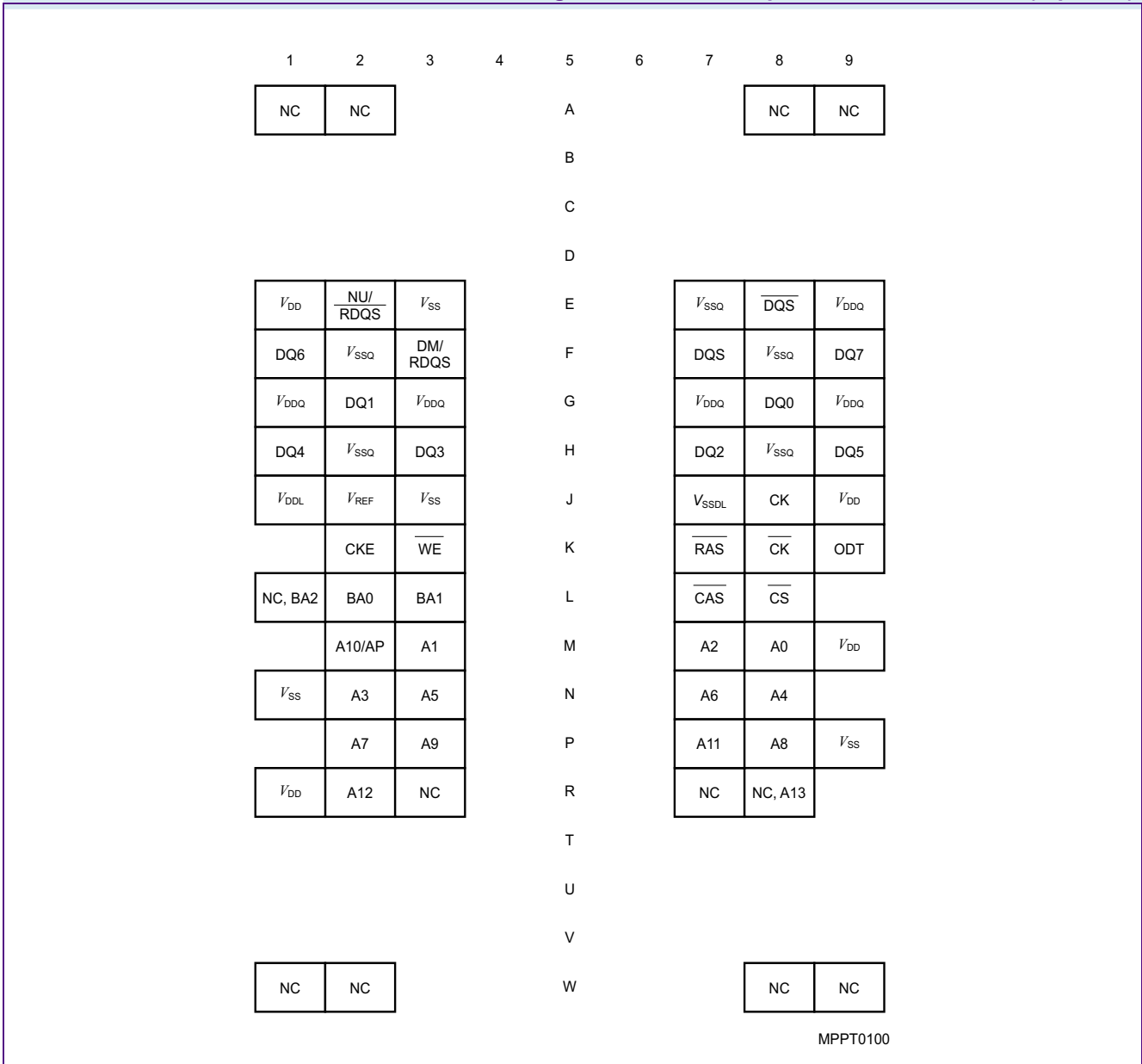
FIGURE 1 Ball Configuration for ×8 components, PG-TFBGA-68 (top view)
