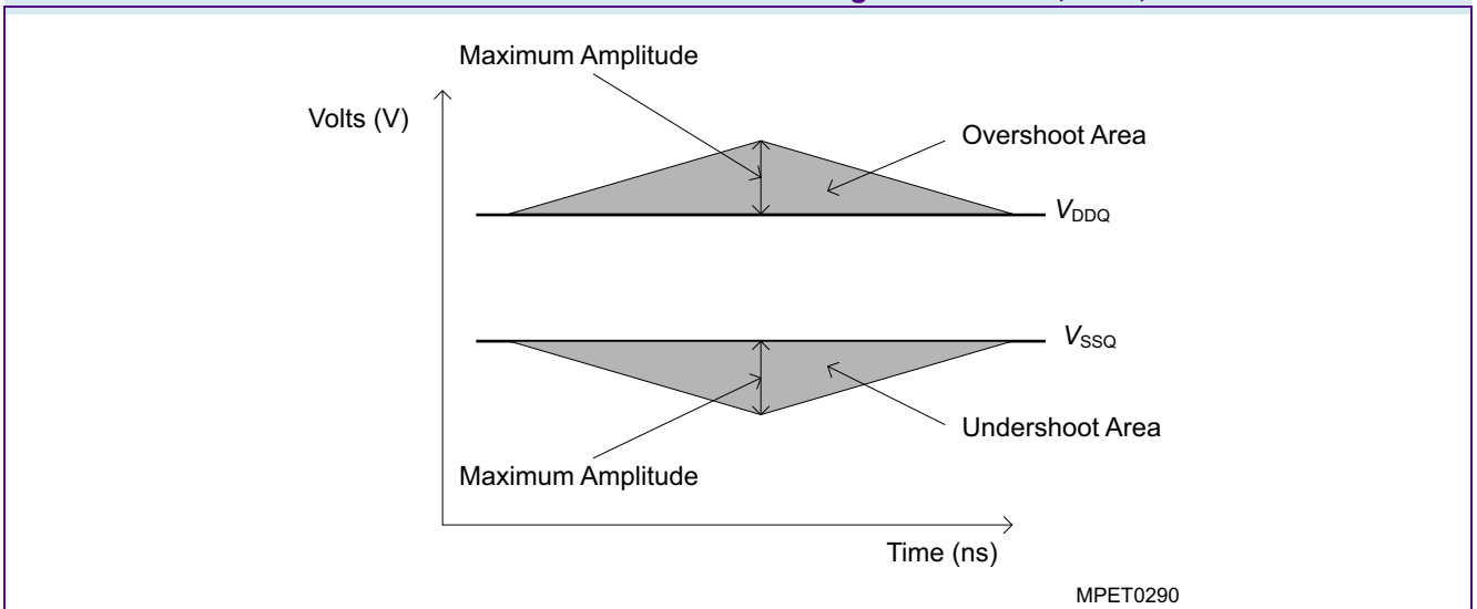
FIGURE 6 AC Overshoot / Undershoot Diagram for Clock, Data, Strobe and Mask Pins
