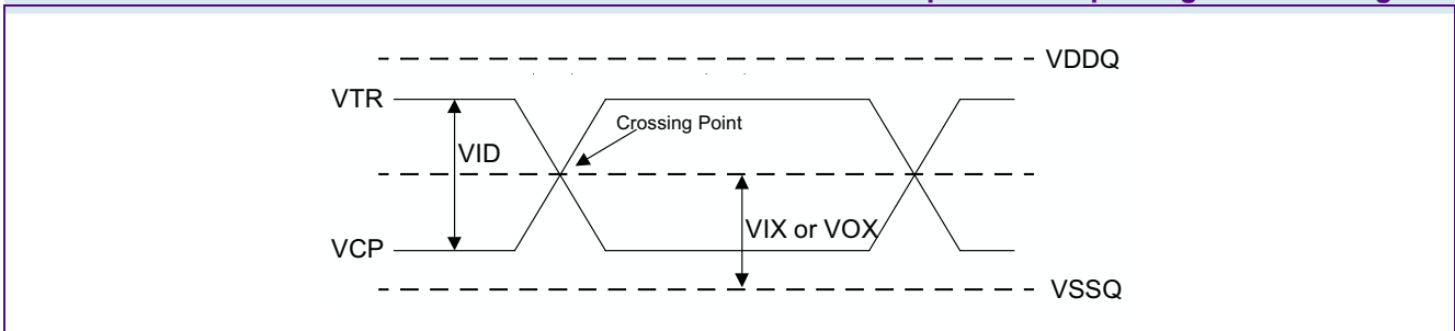
Differential DC and AC Input and Output Logic Levels Diagram
