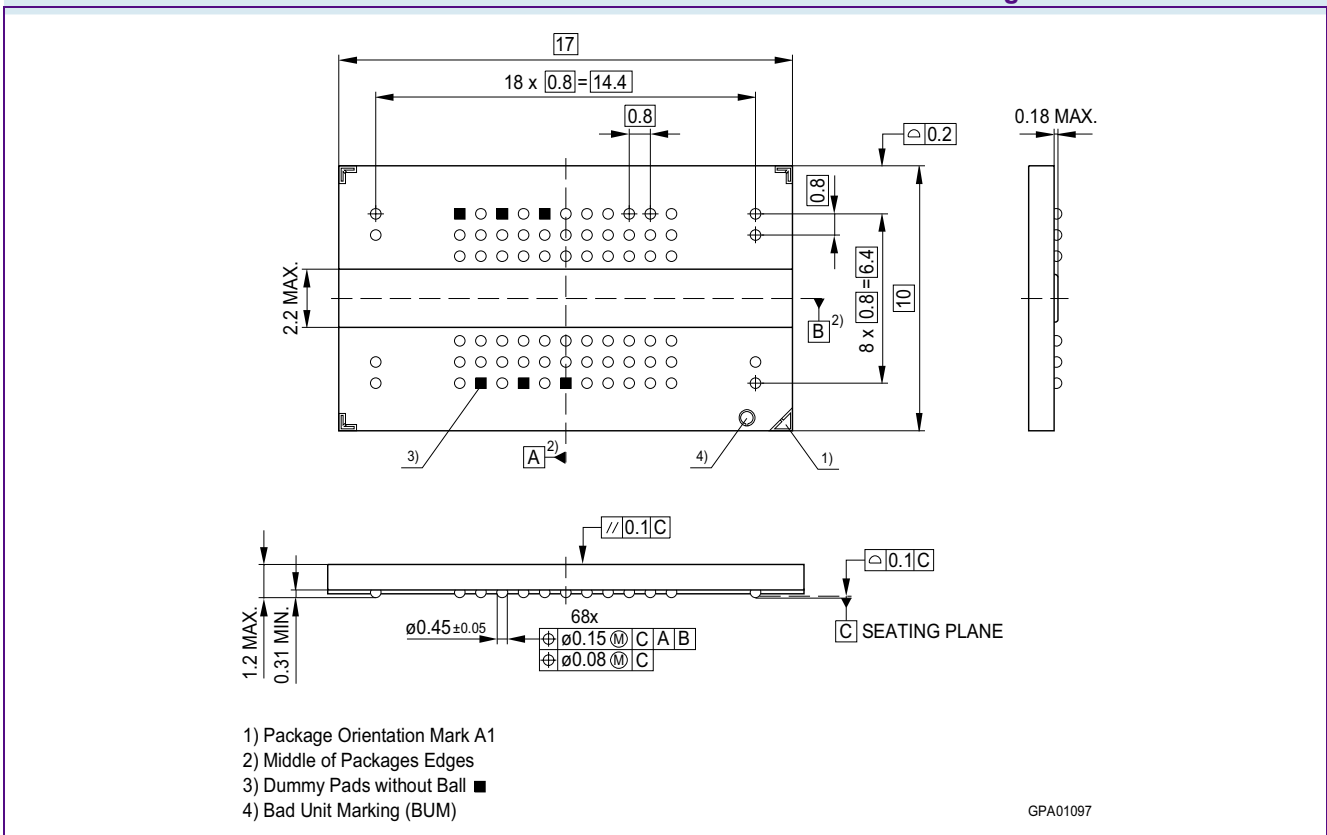
FIGURE 10 Package Outline PG-TFBGA-68
