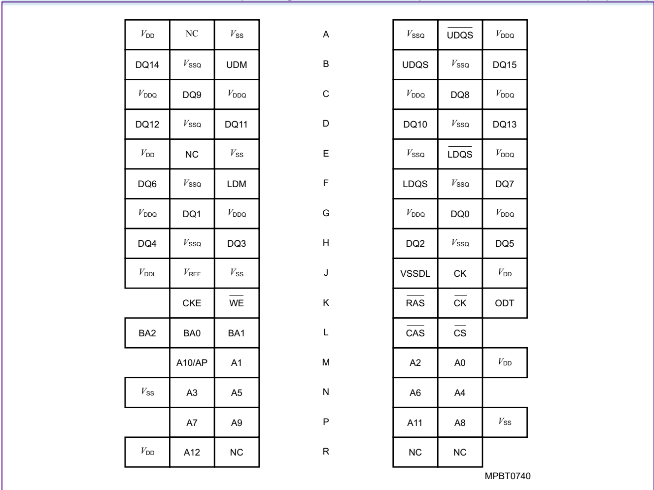
Chip Configuration for x16 Components in PG-TFBGA-84 (Top view)
