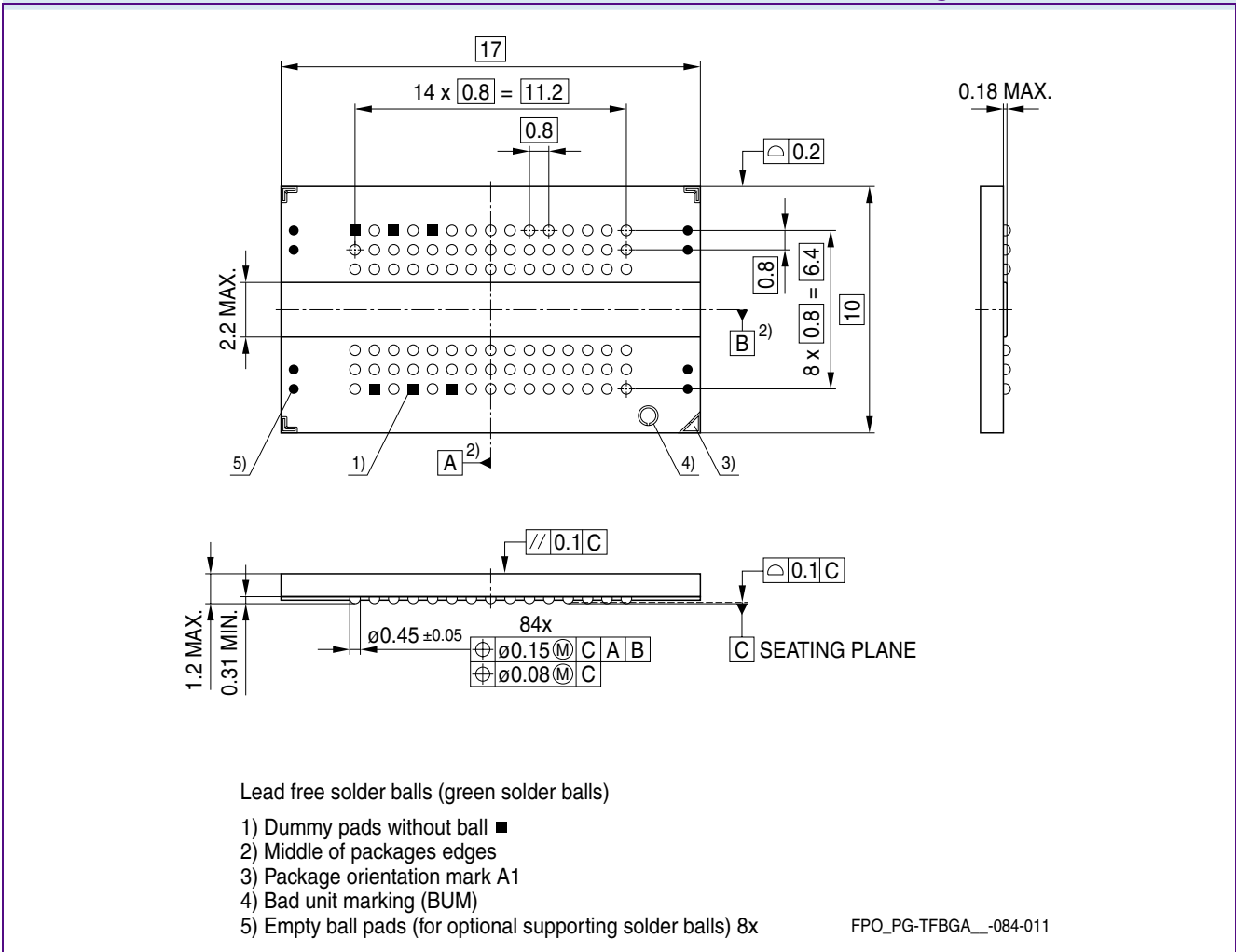
FIGURE 11 Package Outline PG-TFBGA-84
