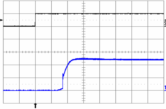
Fig. 1.2V.3: Turn-on transient at full rated load current (resistive) with no output capacitor at V_{in} = 48\text{ V} , triggered via ON/OFF pin. Top trace: ON/OFF signal (5 V/div.). Bottom trace: output voltage (0.5 V/div.). Time scale: 1 ms/div.
