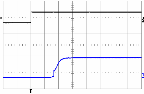
Fig. 1.8V.3: Turn-on transient at full rated load current (resistive) with no output capacitor at V_{in} = 48\text{ V} , triggered via ON/OFF pin. Top trace: ON/OFF signal (5 V/div.). Bottom trace: output voltage (1 V/div.). Time scale: 1 ms/div.
