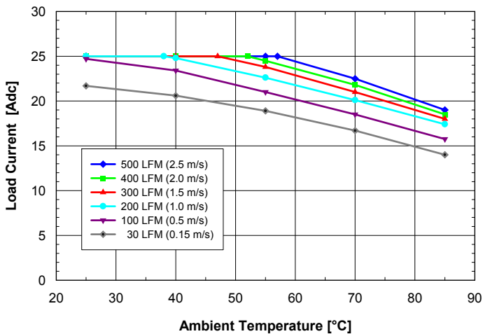
Fig. 1.8V.1: Available load current vs. ambient air temperature and airflow rates for SQM48T25018 converter with D height heat pins mounted vertically with air flowing from pin 3 to pin 1, MOSFET temperature \leq 120^\circ\text{C} , V_{in} = 48\text{ V} .
