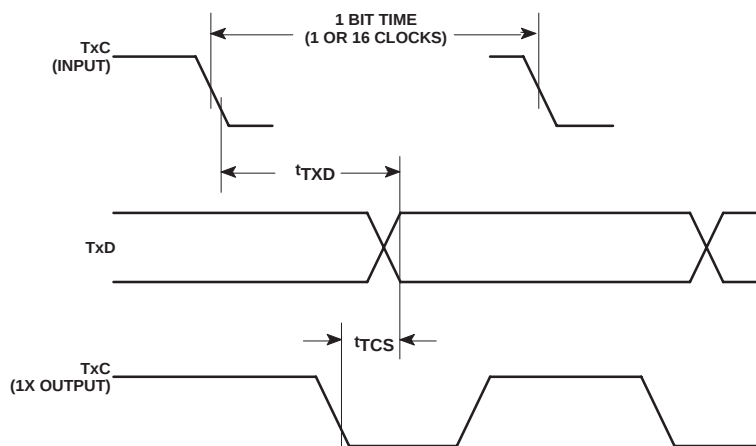
Figure 8. Transmit
