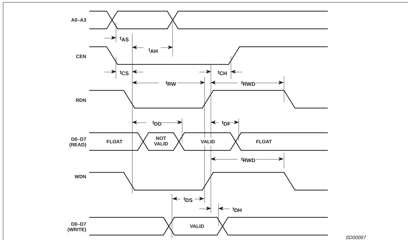
Figure 4. Bus Timing
