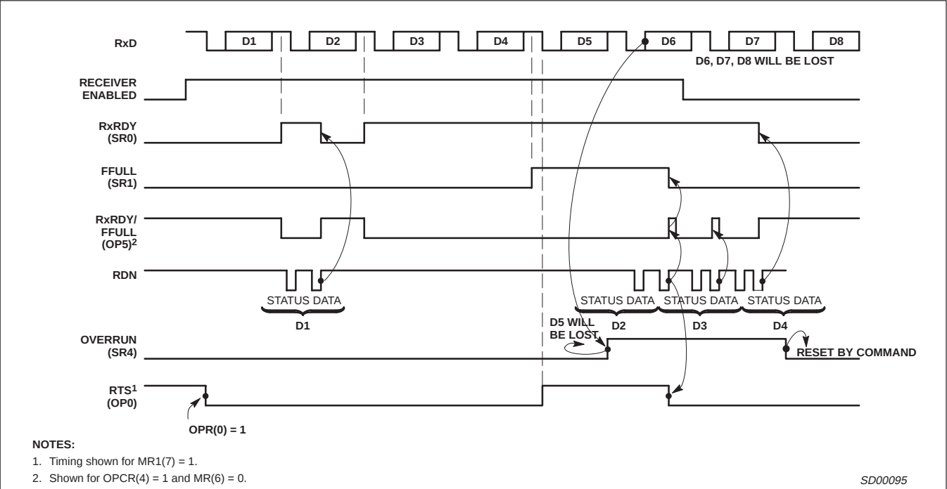
Figure 11. Receiver Timing
