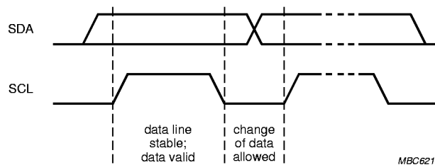
Fig.11 Bit transfer.
