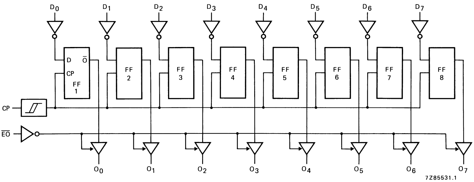
Fig.3 Logic diagram.
