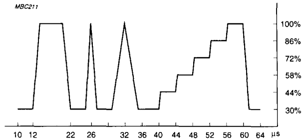
Fig.12 Test signal waveform.
