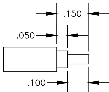
STRIPPING DIMENSIONS
