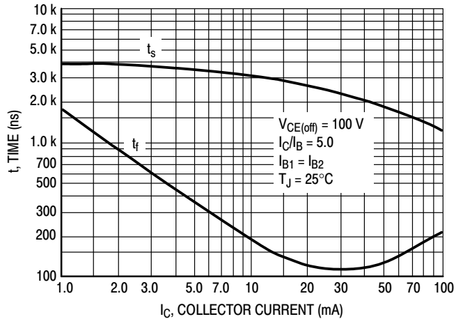
Figure 7. Turn-Off Time
