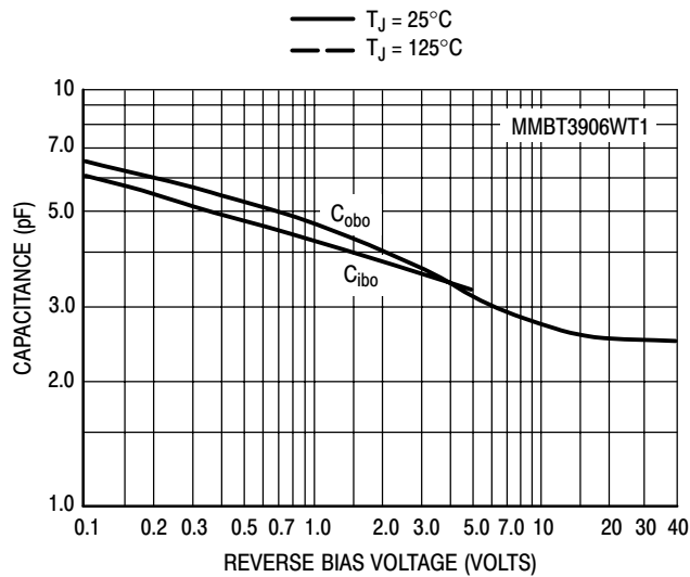
Figure 32. Capacitance
