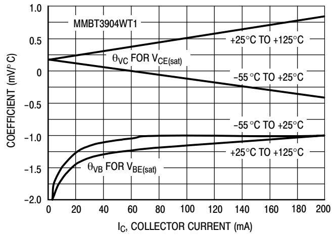
Figure 16. Temperature Coefficients
