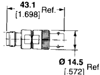
Part No. 1057845-1 M/A-COM Model No. 3180-2320-00
