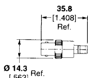
Part No. 1058077-1 M/A-COM Model No. 3282-2223-00
