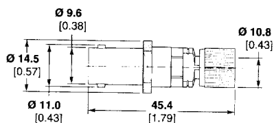
Part No. 1-1393665-7
