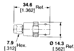
Part No. 1058083-1 M/A-COM Model No. 3282-2241-00
