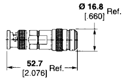
Part No. 1057392-1 M/A-COM Model No. 3082-2321-00
