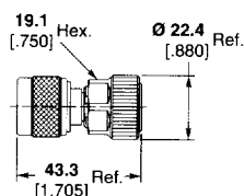
N Series Plug to 7 mm Jack
