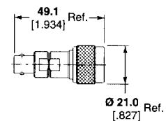
Part No. 1057390-1 M/A-COM Model No. 3082-2320-00
