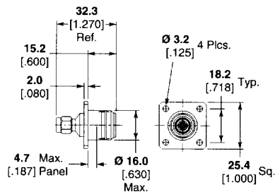
Part No. 1058667-1 M/A-COM Model No. 3682-2243-00
