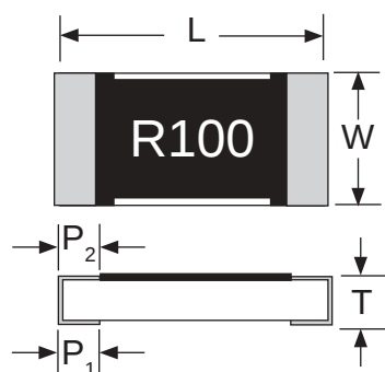
Case Sizes 0402, 0603, 0805, 1206, 2010 & 2512
