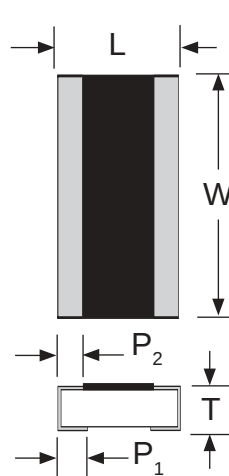
Case Sizes 1225 & 7520
