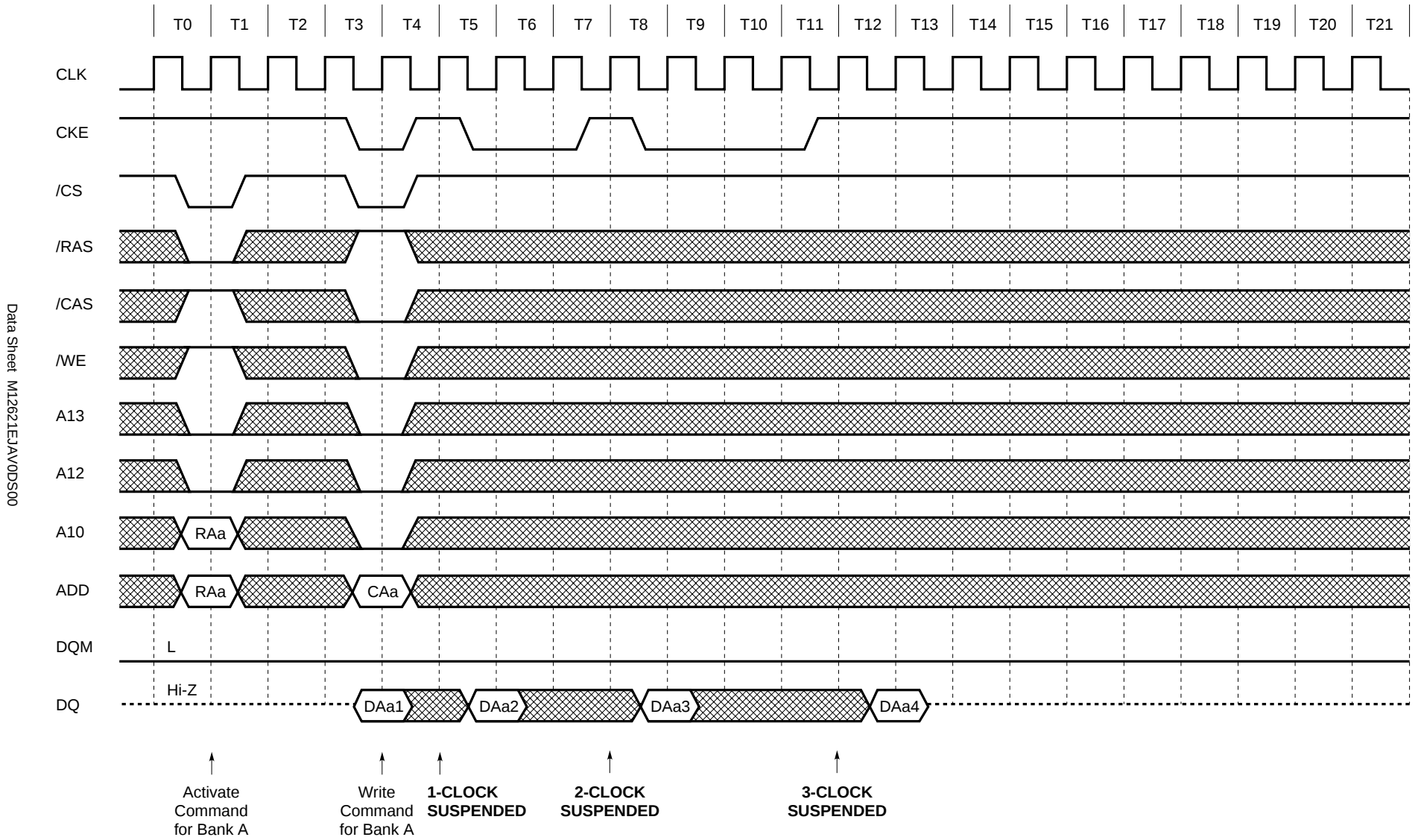
Clock Suspension during Burst Write (using CKE Function) (2/2) (Burst Length = 4, /CAS Latency = 3)
